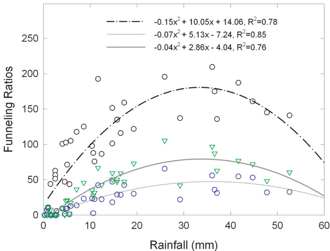
Fig 6. Relationships between event stemflow funneling ratios and rainfall depth for the different canopy types.
