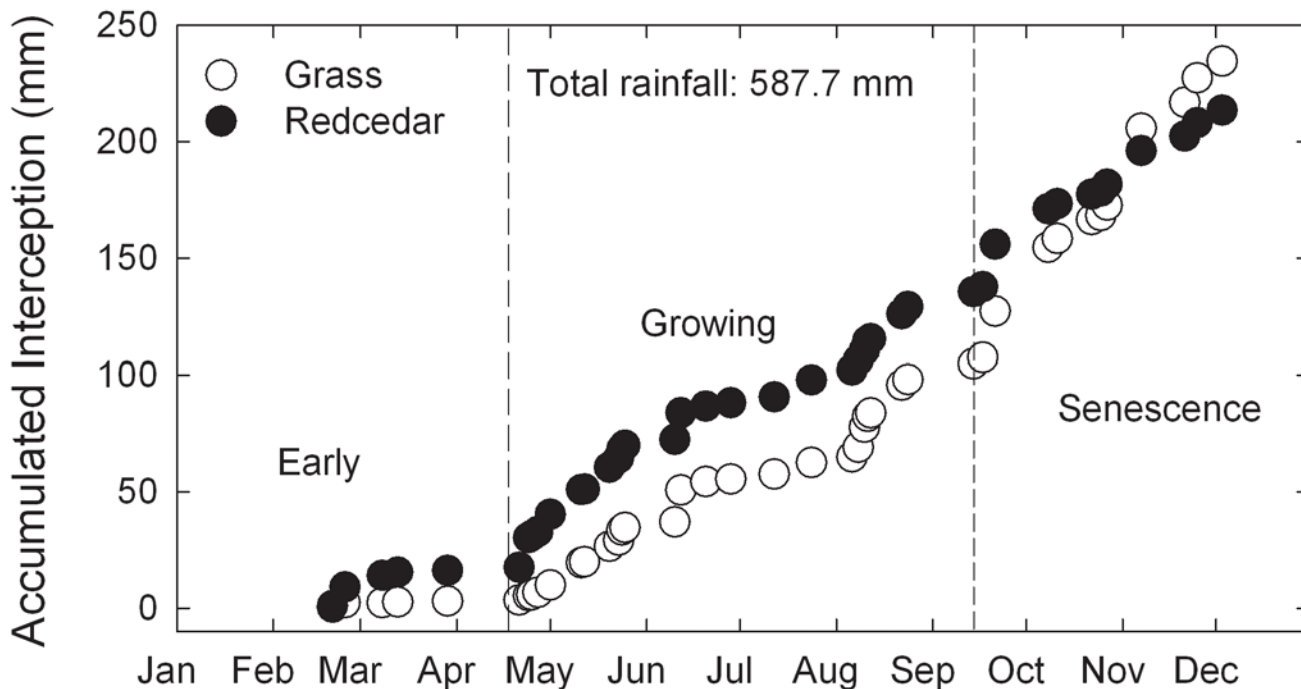
Fig 9. Comparison of accumulated interception loss to tallgrass prairie and redcedars.
