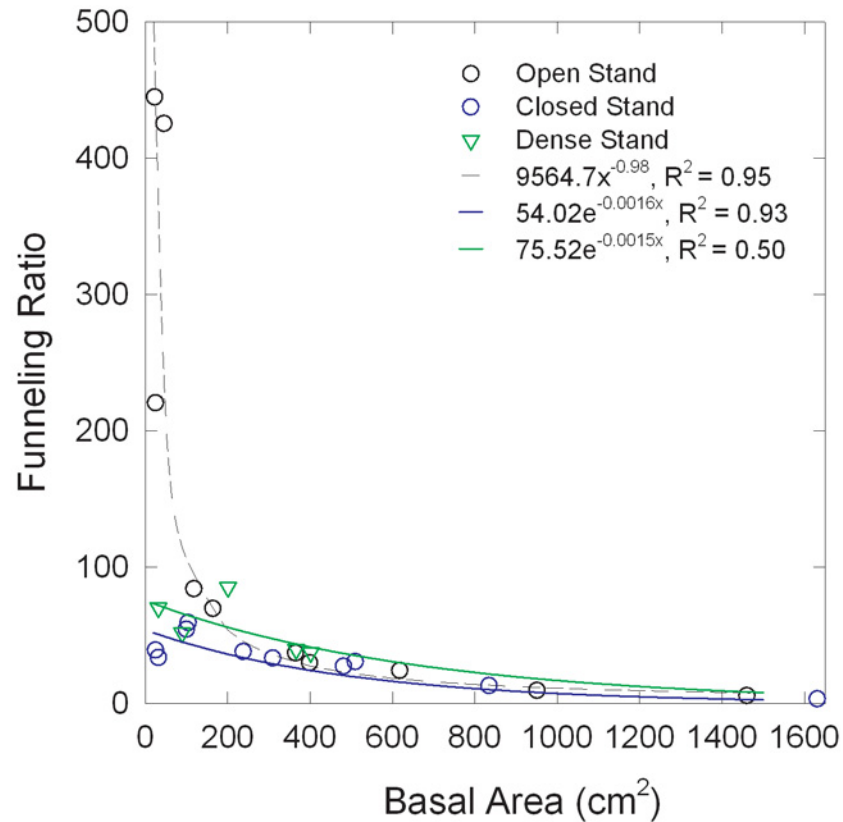
Fig 5. Relationship between annual stemflow funnelling ratios and redcedar basal area for the different canopy types.
