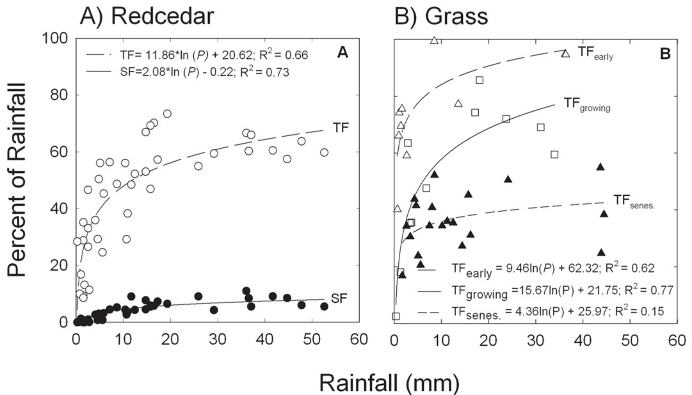
Fig 3. Non-linear models describing average throughfall (TF) ratios and stemflow (SF) ratios for redcedar trees (A) and TF for tallgrass prairie vegetation at different growing stages (B) under the range of event rainfall sizes.
