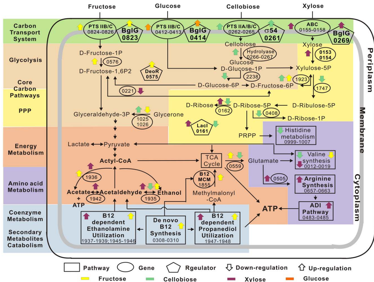
Figure 6. Cellular model of the Thermoanaerobacter glycometabolism. Key transport, metabolic and regulatory genes and pathways are illustrated. Yellow arrows: genes specifically expressed under fructose (glucose as reference). Green arrows: those specifically expressed under cellobiose (glucose as reference). Purple arrows: those specifically expressed under xylose (glucose as reference). Orange arrows: the two putative operons specifically expressed under glucose but downregulated under all other substrates. Up arrow: upregulation; down arrow: downregulation. IDs of the corresponding genes in X514 are shown. doi:10.1371/journal.pgen.1002318.g006
