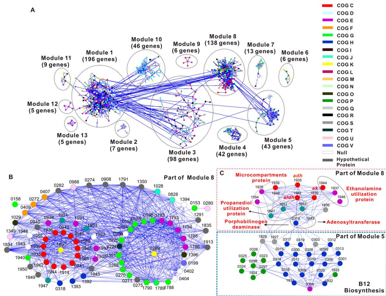
Figure 3. Gene co-expression network of the Thermoanaerobacter glycobiome . A) Global view of the network. B) A sub-module of Module 8. Only those genes known to be involved in xylose catabolism and their first neighbors (genes directly connected to xylose catabolism genes) in the network are shown. C) The sub-network that includes genes directly involved in B 12 synthesis and ethanol fermentation. It includes components from both Module 5 and Module 8. Each node represents a gene, which is color-coded using its predicted COG-based functional classification ( http://www.ncbi.nlm.nih.gov/nuccore/NC_010320 ; NC_010320.1 ). Any two genes with a Pearson correlation \geq 0.94 in their expression patterns are connected (via edges, which are shown as lines; blue lines indicate positive correlation). For a given gene, its first neighbors are defined as those gene(s) that are directly connected to it. doi:10.1371/journal.pqen.1002318.g003
